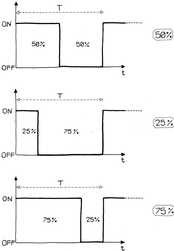
Figure 5-3. PWM in action
