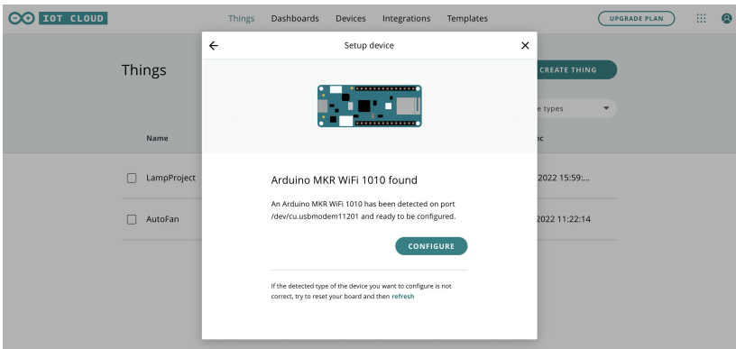
Figure 7-3. Connecting an Arduino to the IoT Cloud
