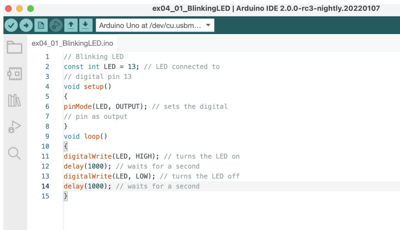
Figure 4-2. The Arduino IDE with your first sketch loaded
