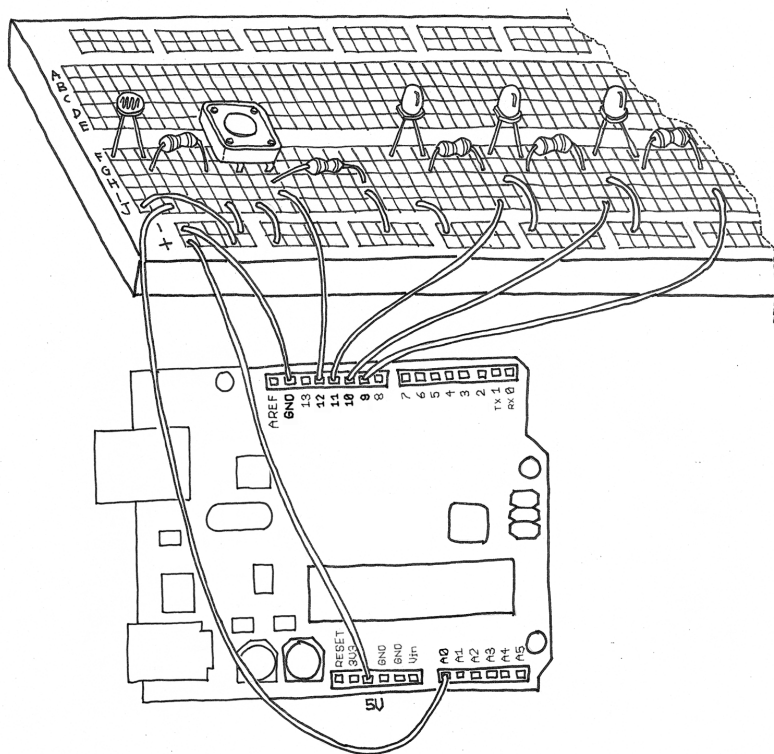
Figure 6-2. The Arduino Networked Lamp circuit
