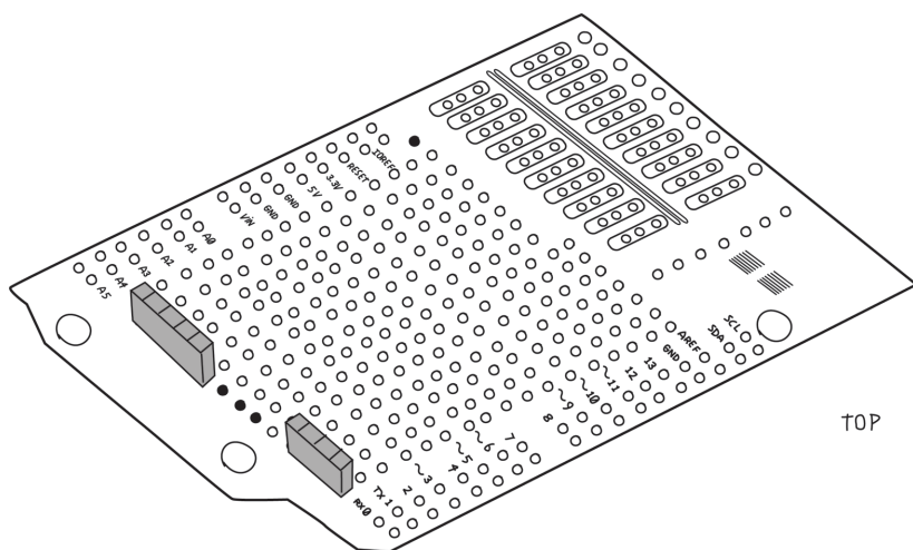
Figure 8-19. A four position socket for the DHT11 sensor and a five position female header for the RTC
