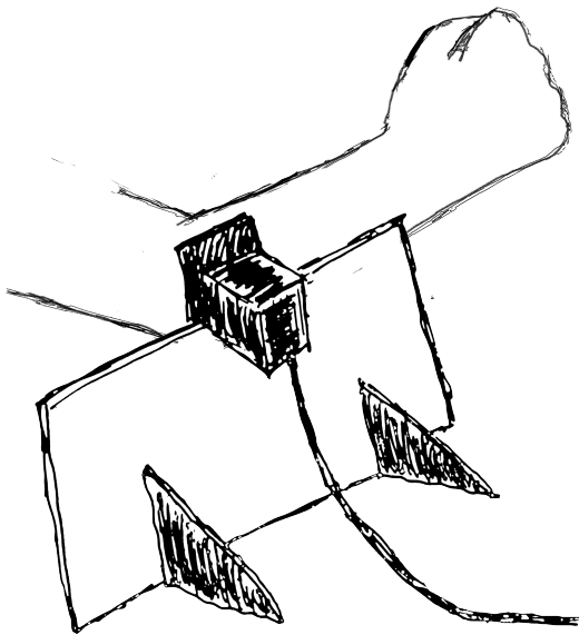
Figure 10-3. Cardboard arm with fist attached to servo motor
